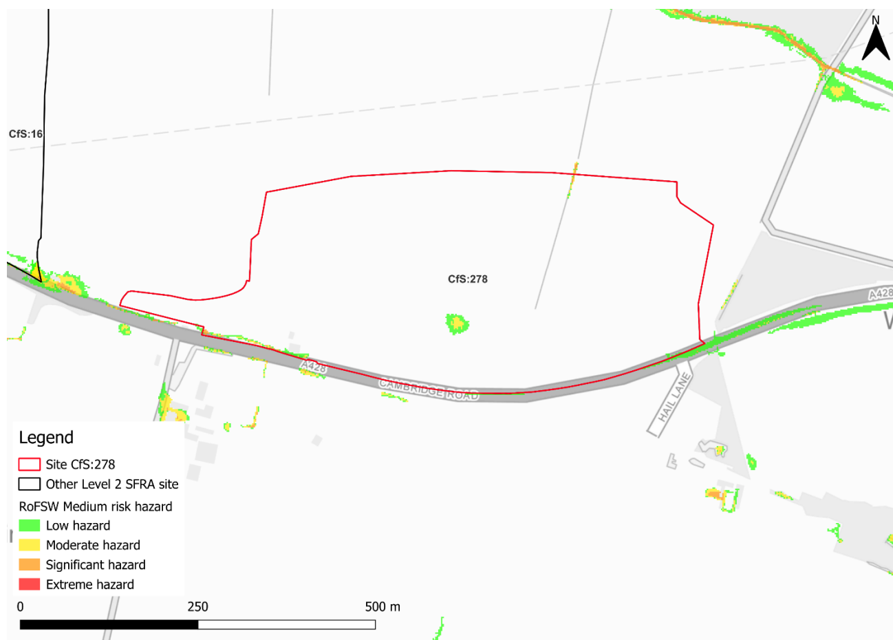
Figure 3-3: High risk event surface water flood hazard 1 (Third generation - Risk of Flooding from Surface Water map)
