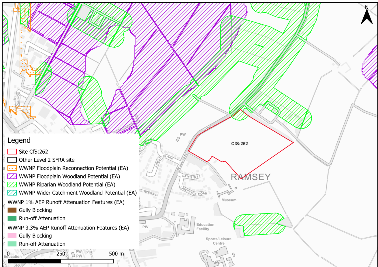
Figure 2-1: Natural Flood Management (NFM) potential mapping
