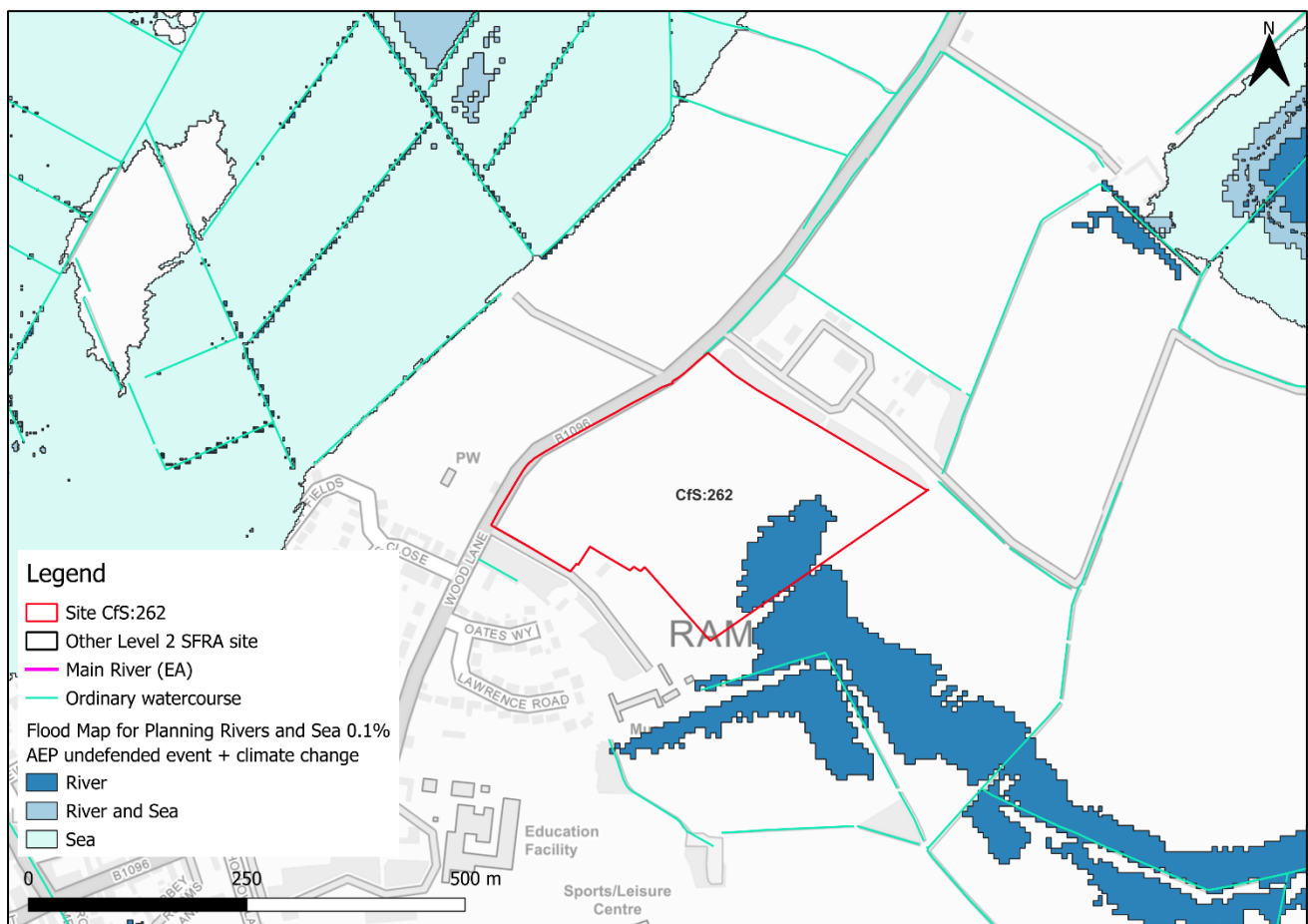
Figure 2-2: Flood Map for Planning 0.1% AEP (fluvial and tidal) undefended flood event +6% (central climate change allowance)
